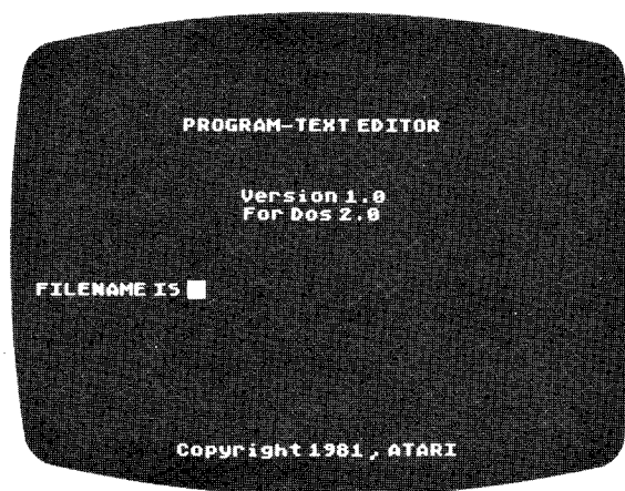
Figure 2 Filename Prompt
