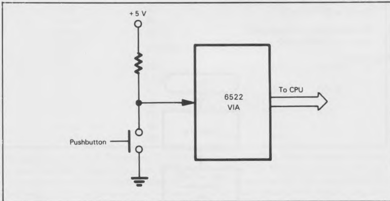
Figure 11-14. A Pushbutton Circuit
