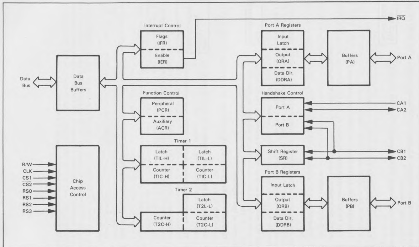
Figure 11-8. Block Diagram of the 6522 Versatile Interface Adapter
