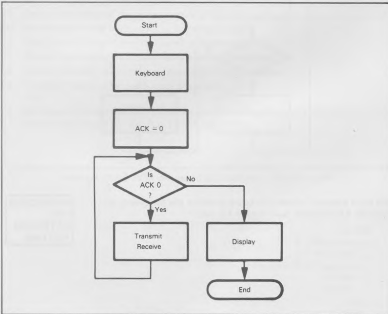
Figure 13-19. Initial Flowchart for Transaction Terminal
